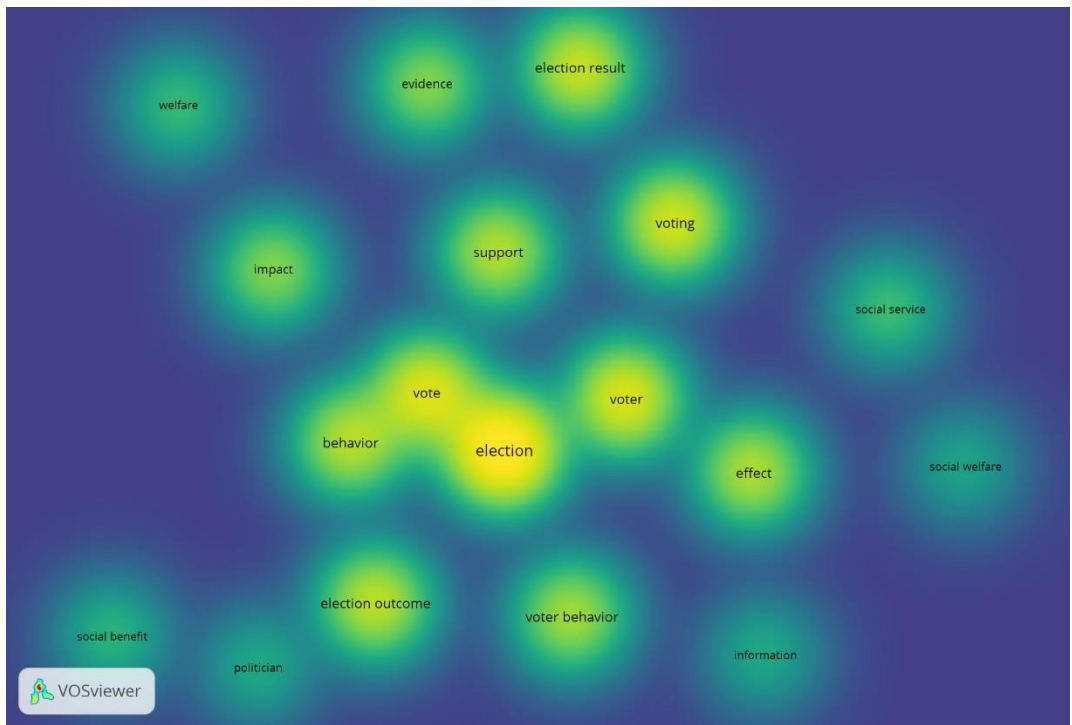
Figure 4. Visualization of density in GS data base
